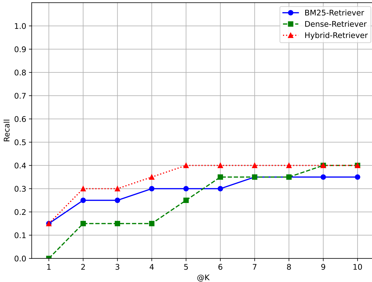
Query 19
